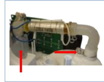
Loosen the heating element left and right and take it out
